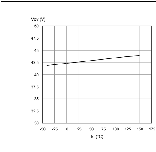
Figure 11. Overvoltage shutdown
